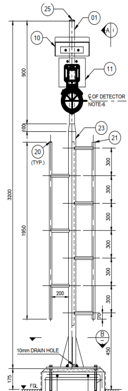
Flame Detector Stand with Ladder
